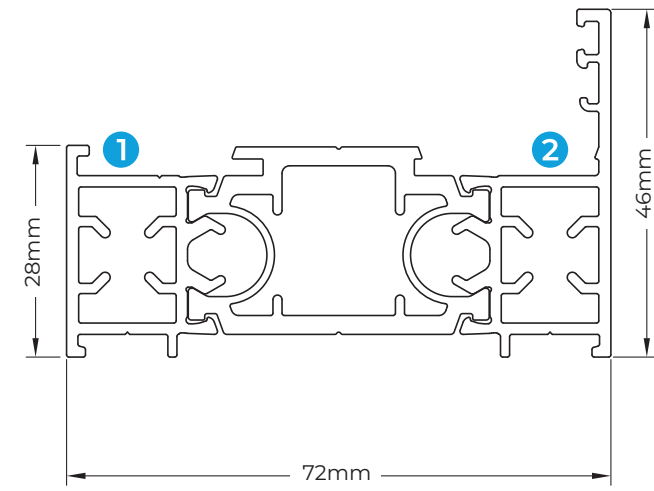
SP100 SMALL OUTER FRAME
