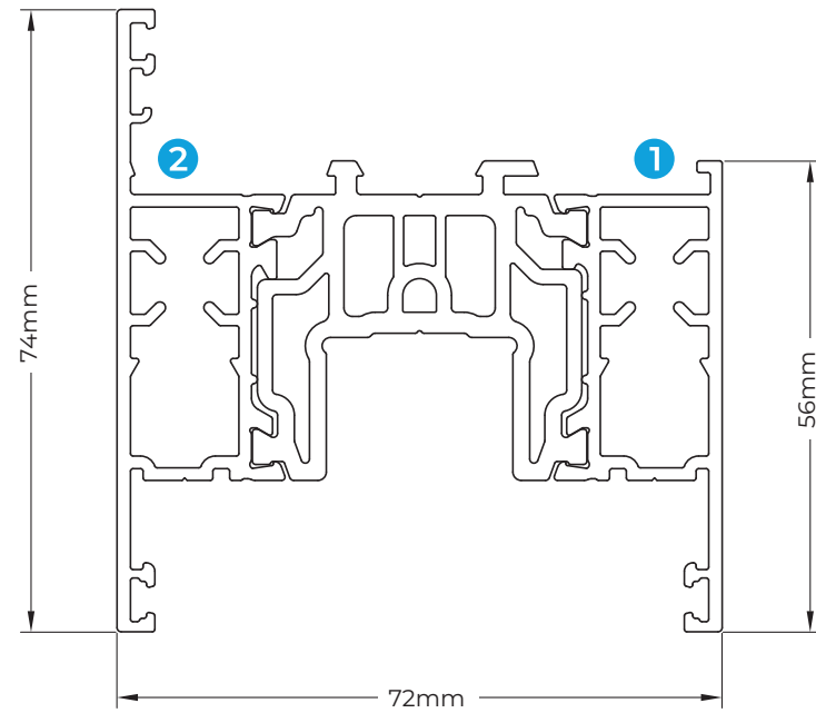
SLS301 CONTEMPORARY SASH
