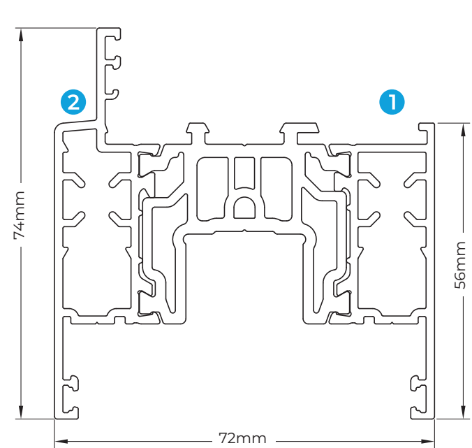
SLS300 STEPPED SASH
