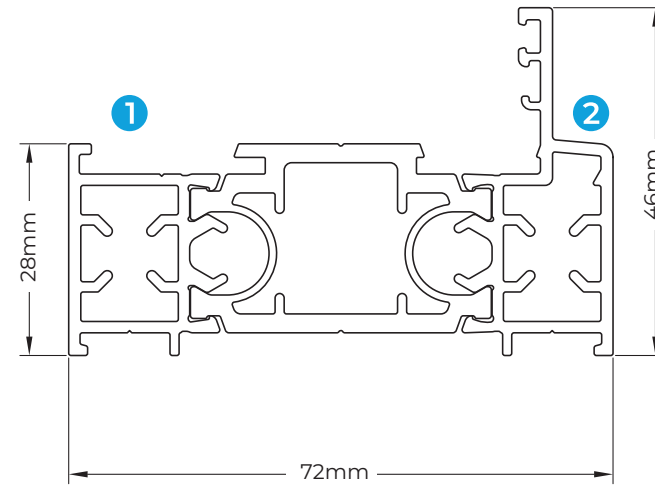
SLS150 SMALL STEPPED OUTER FRAME
