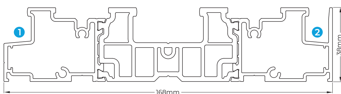
SLS100 2 PANE STANDARD FRAME
