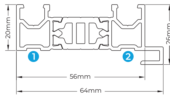
SLS103 JAMB EXTENSION
