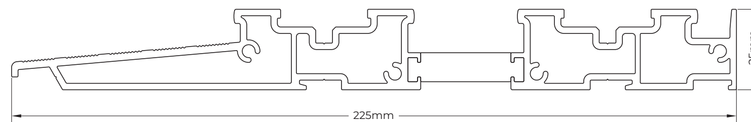
SLS700 LOW THRESHOLD WITH RAMP
