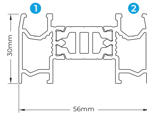
SLS250 4 PANE ADAPTOR
