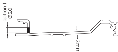
1 SLS013 TWIN TRACK DRAINAGE TRAY BLACK ONLY
