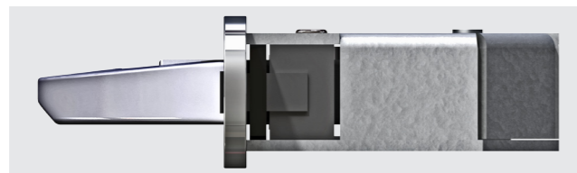
Special design tensile steel chamfered hook allows a high degree of fitting tolerance for door installation.
