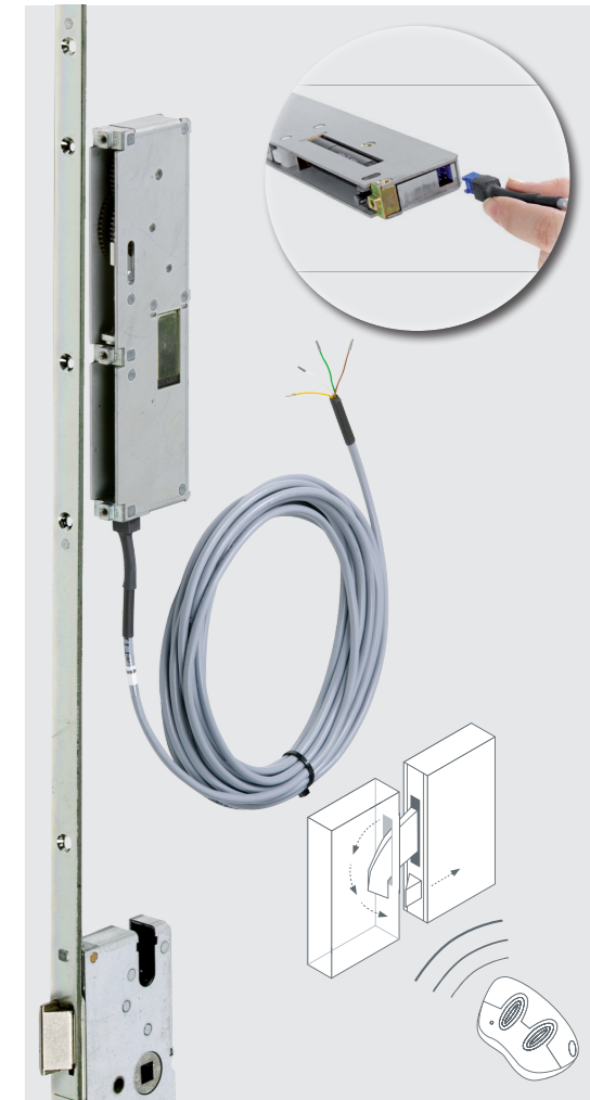
Easy upgrade to electronic operation via screw-on 12v Motor. Fully compatible with existing intercom, 'electronic' door closers and other access control systems.
